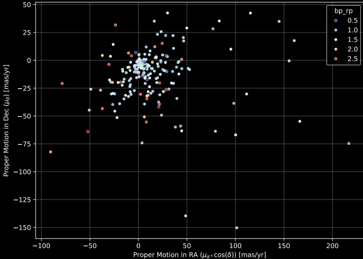
APOGEE DR17 Field: [K2_C8_137-61_btx] Proper Motion Diagram (n= 200)
