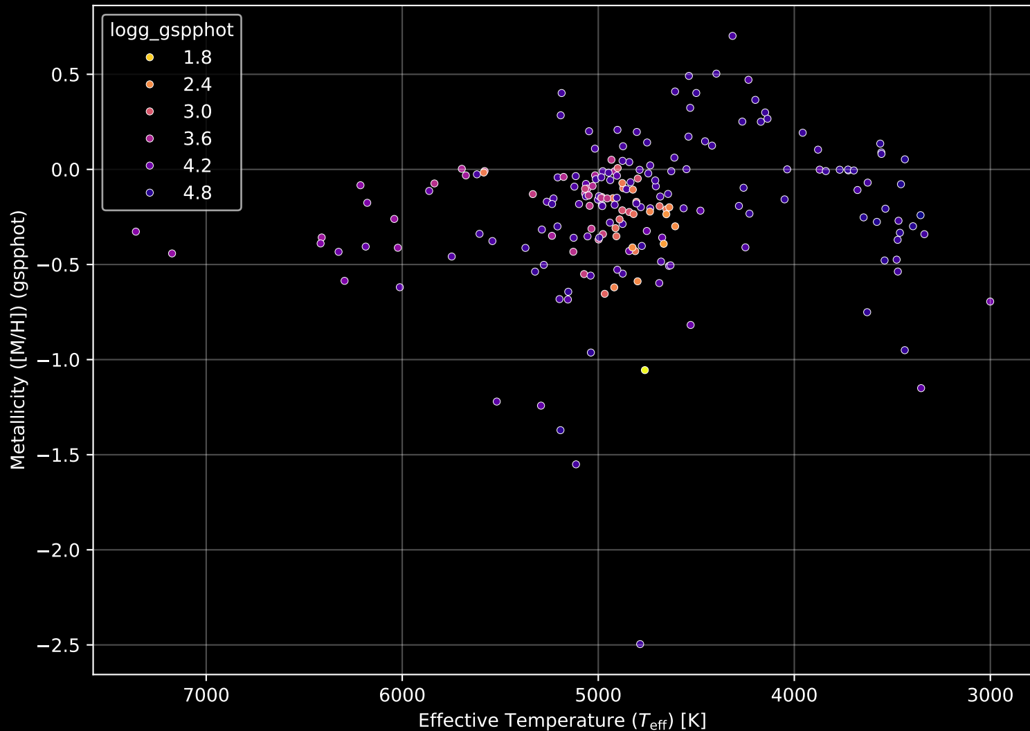
APOGEE DR17 Field: [K2_C8_137-61_btx] Stellar Population Parameters (n= 200)
