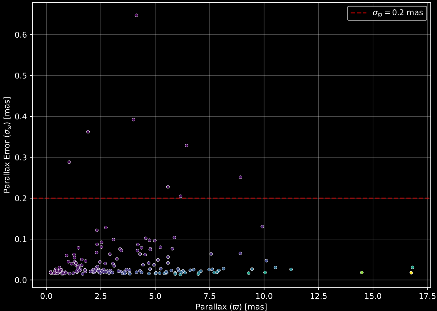
APOGEE DR17 Field: [K2_C8_137-61_btx] Parallax Quality (n= 200)
